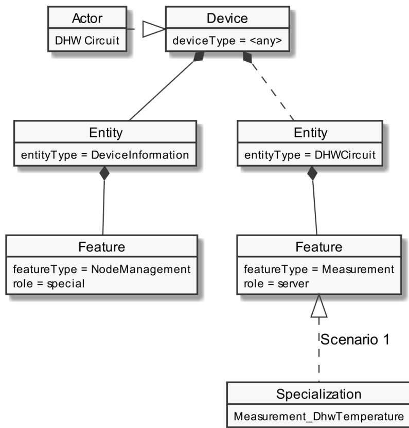
Figure 4: Actor "DHW Circuit" overview
